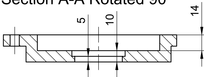
Section A-A Rotated 90°
